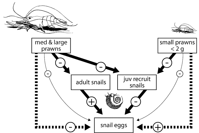
Fig. 8. Proposed trophic interactions between large or small prawns and adult snails, snail recruits, and snail eggs. Large prawns have negative direct and indirect effects on all snail life stages. On the other hand, small prawns (<2 g) are limited in their ability to kill adult snails. A negative effect of juvenile recruit snails on eggs (due to competitive or egg-cannibalistic effects) led to positive indirect effects of small prawns on snail eggs, despite a strong negative effect on snail recruitment.
